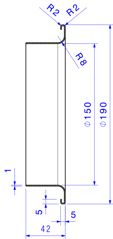
Section view POS 1
